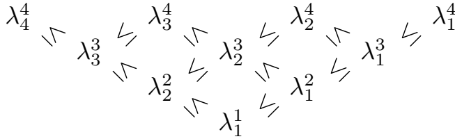
FIGURE 1. Interlacing array of eigenvalues of all principal corners of a 4 \times 4 matrix.
